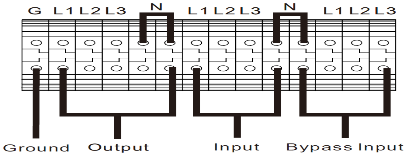
Terminal block wiring diagram for 33 HV10K(L)/15K(L)/20K(L)
