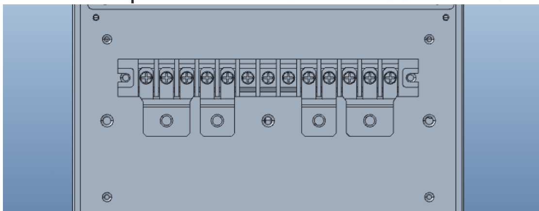
31 HV10K(L)/15K(L)/20K(L) and 31 LV 5K(L)/7.5K(L)/10K(L) schematic diagram for connection of short circuit sheet copper
