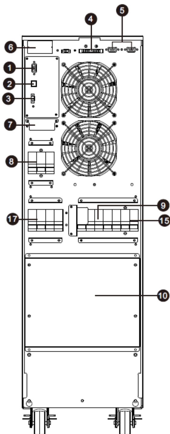
Diagram 1: HV 10K(L)/15K(L)/20K(L) pannello posteriore
