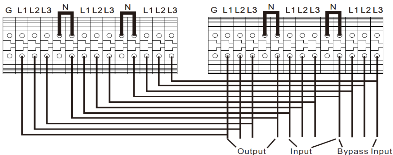
Wiring diagram of parallel system for 33 HV10K(L)/15K(L)/20K(L)
