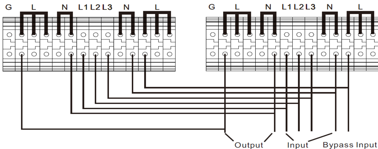
Wiring diagram of parallel system for 31 HV10K(L)/15K(L)/20K(L)
