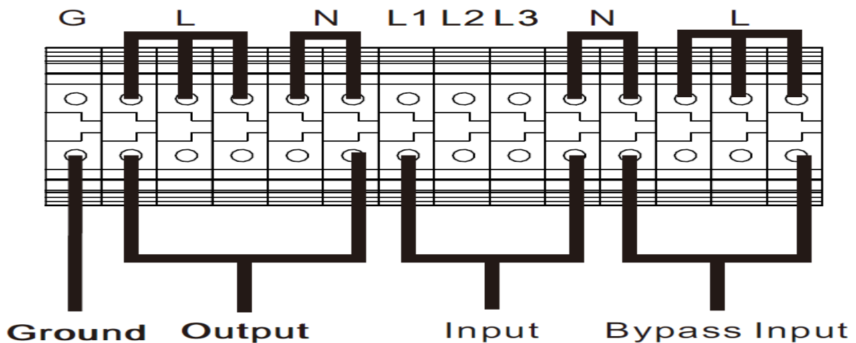
Terminal block wiring diagram for 31 HV10K(L)/15K(L)/20K(L)
